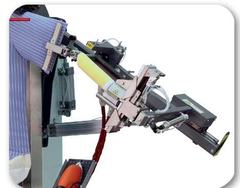
SHORT SLEEVE CLAMPS DEVICE
